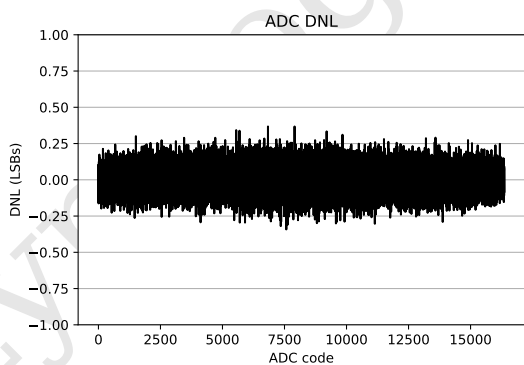
(a) DNL
