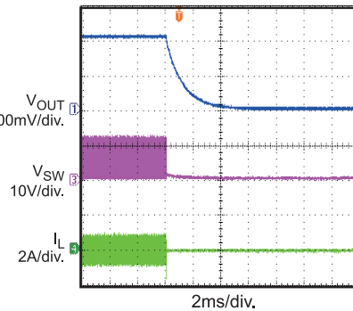
Thermal Shutdown
