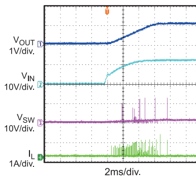
Start-Up Through VIN I_{OUT} = 0A
