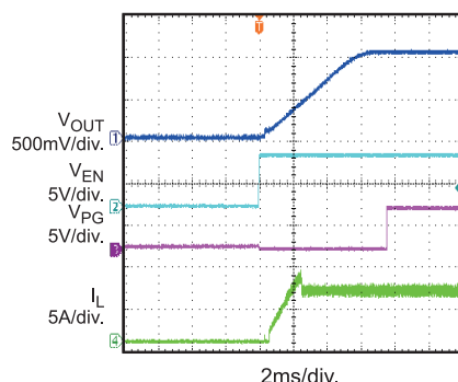
Power Good Through EN Start-Up I_{OUT} = 6A
