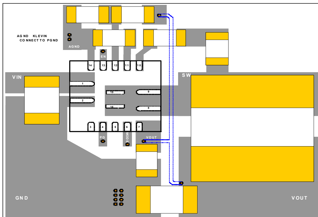
Figure 15: Recommend Layout
