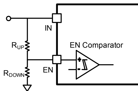
Figure 9: Adjustable UVLO
